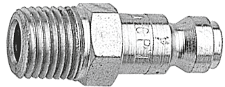
Tru-Flate 1/4" Series NPT Male Pipe Thread
