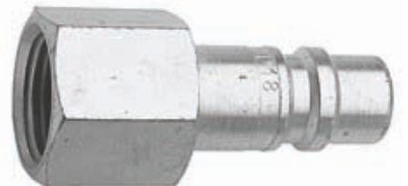
1/2" Series NPT Female Pipe Thread
